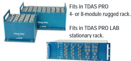
TDAS PRO LAB SIM and TDAS PRO SIM (13.7 x 12.2 x 3.4 cm) are standalone data recorders with 8 fully-programmable sensor input channels that work with a variety of sensors.
